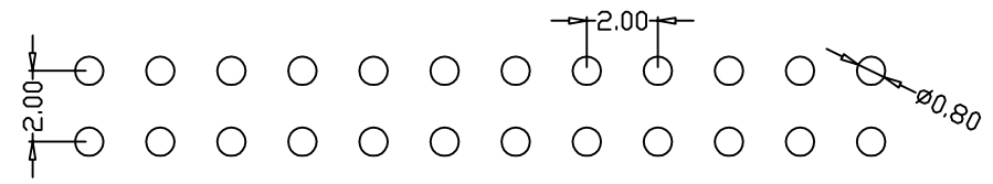
P. C. B LAYOUT
